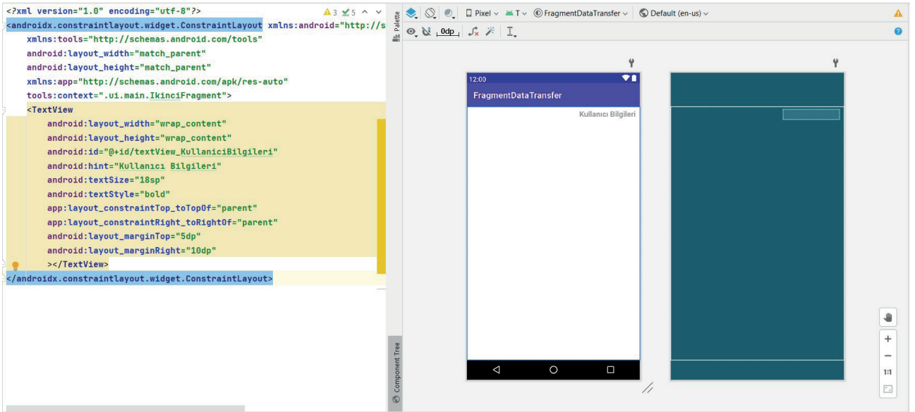
Görsel 6.63: FragmentDataTransfer fragment_ikinci.xml
